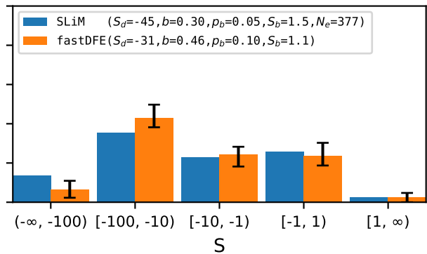
Frequent beneficial
