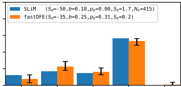
Weakly deleterious
