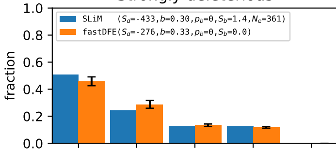
Strongly deleterious
