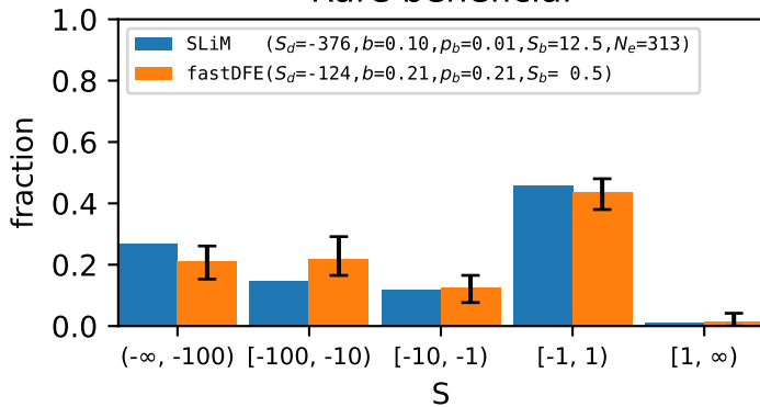
Rare beneficial
