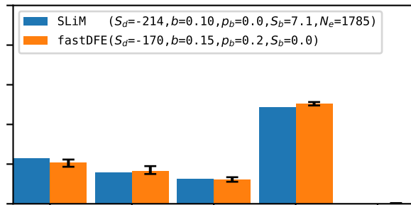
Weakly deleterious
