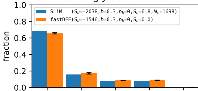
Strongly deleterious
