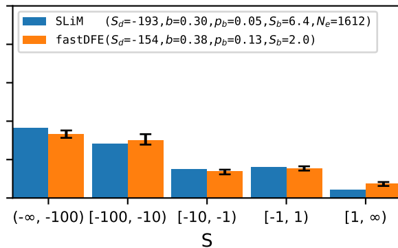
Frequent beneficial
