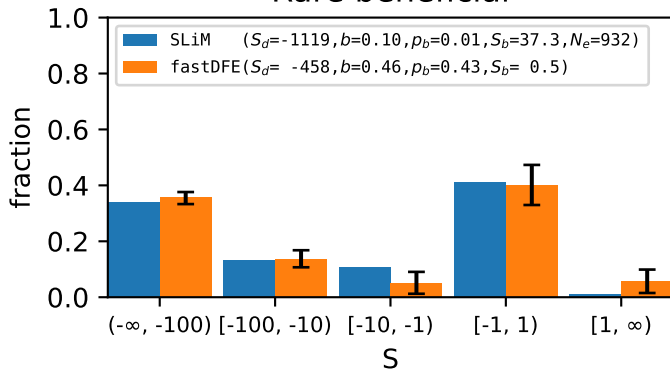
Rare beneficial
