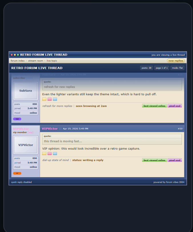
WIDGET PREVIEW
