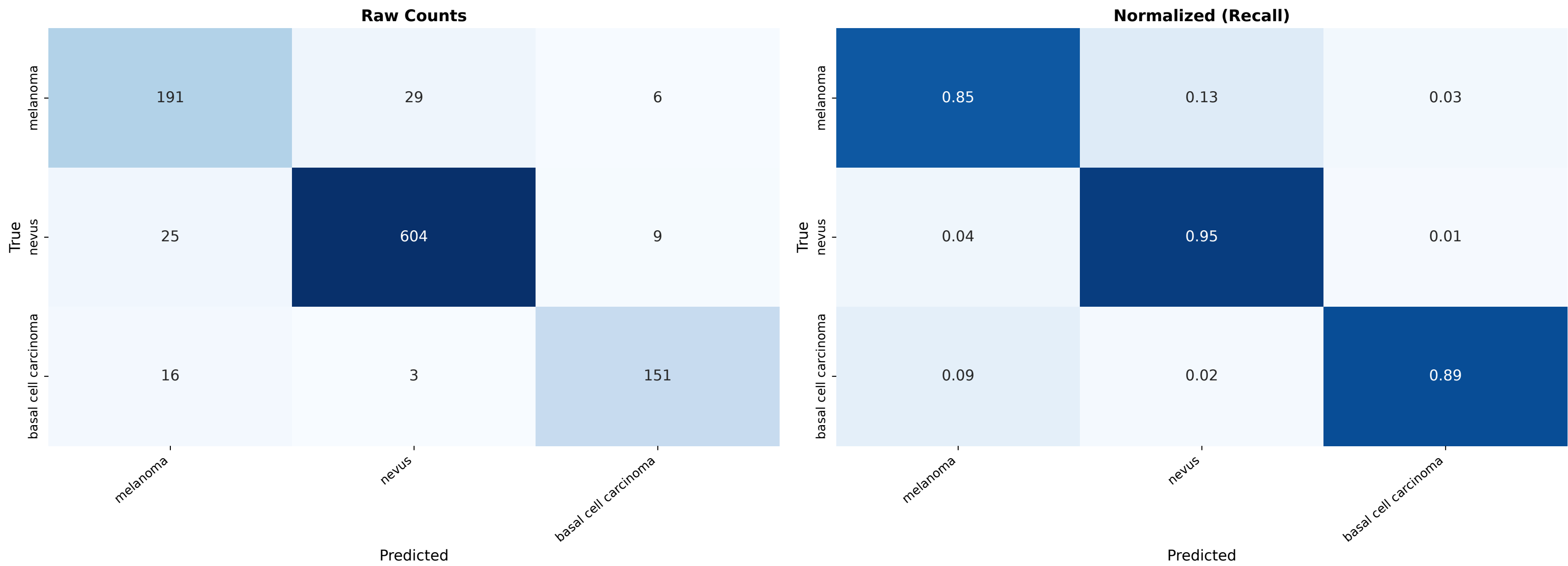
Confusion Matrix - Test
