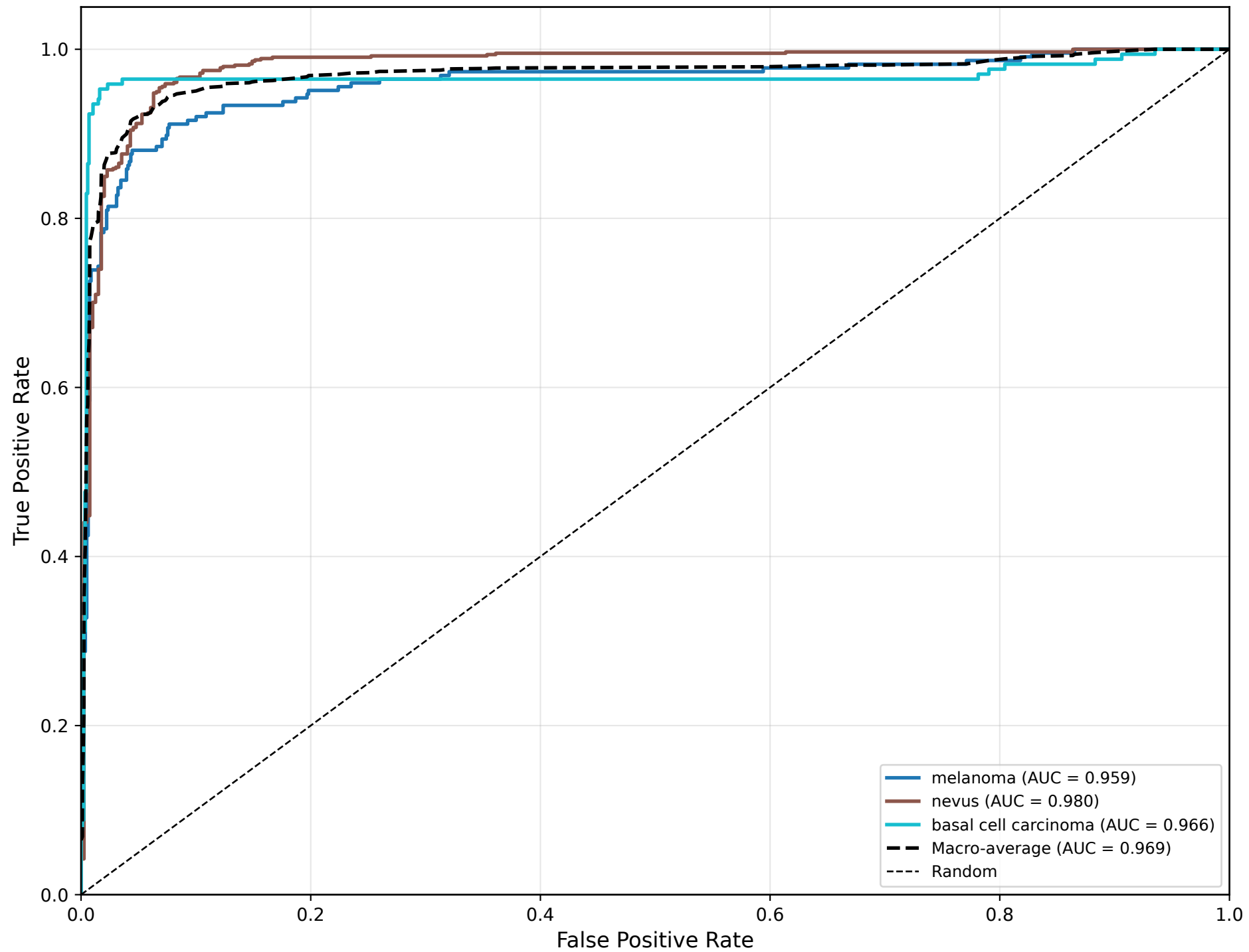
ROC Curves - Test
