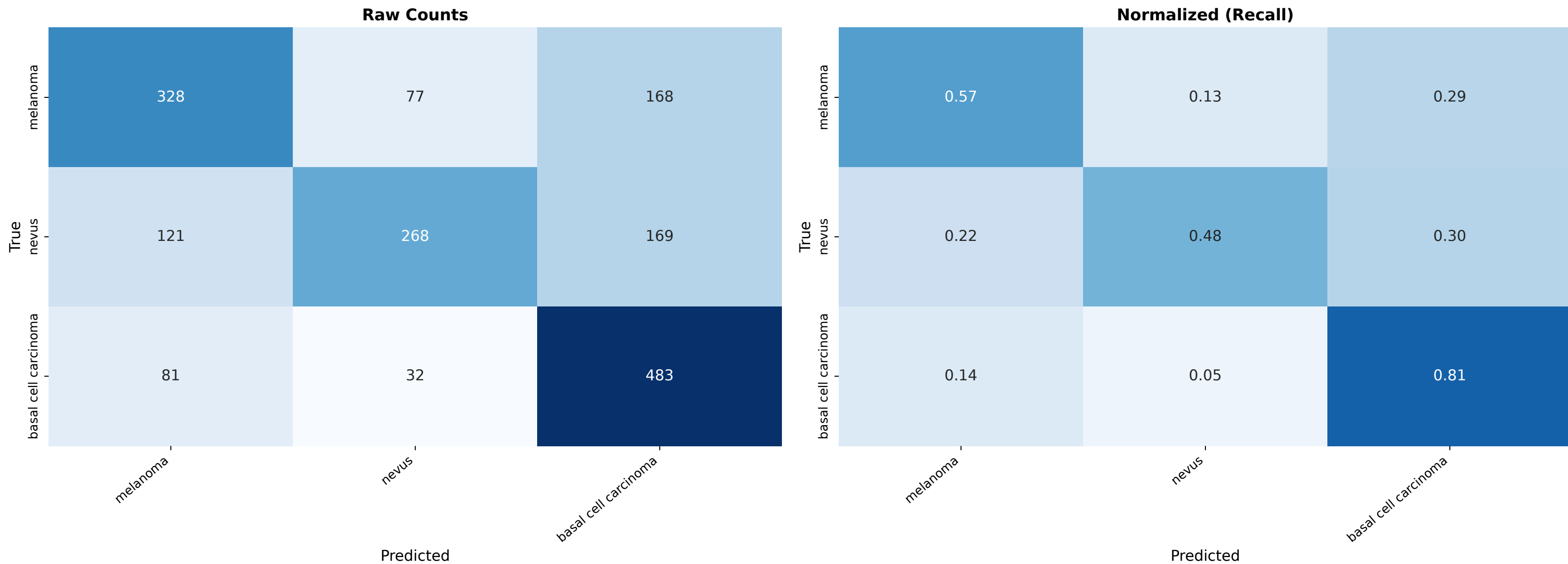
Confusion Matrix - fitzpatrick17k
