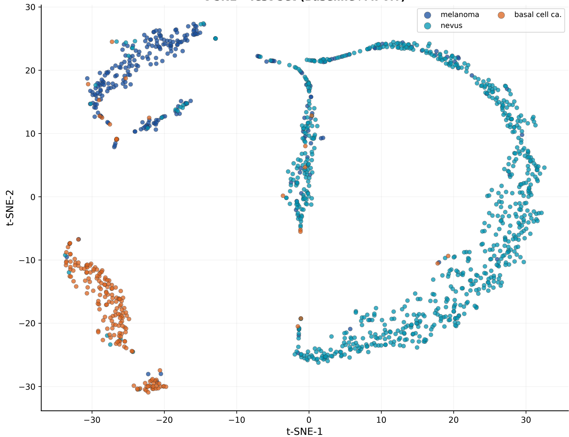
t-SNE - Test Set (Baseline+MI ViT)
