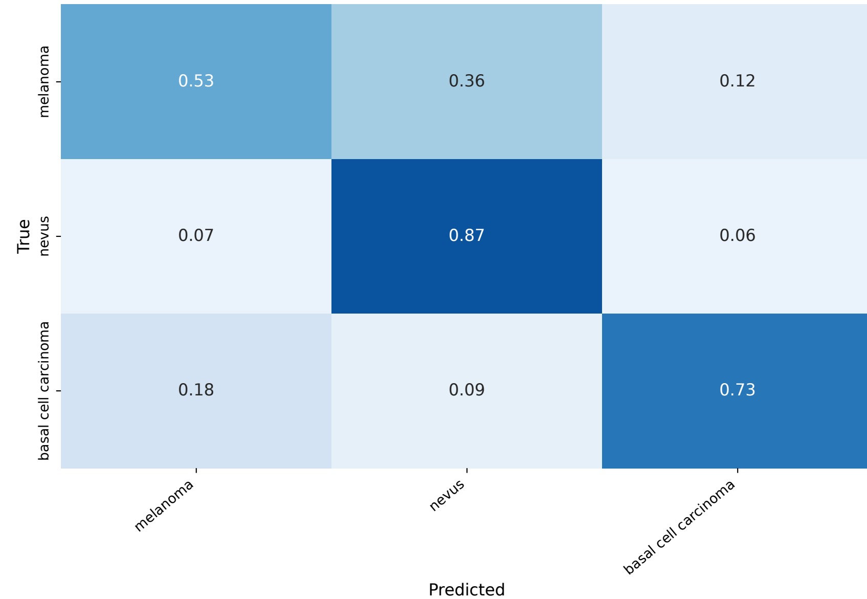
Normalized (Recall)
