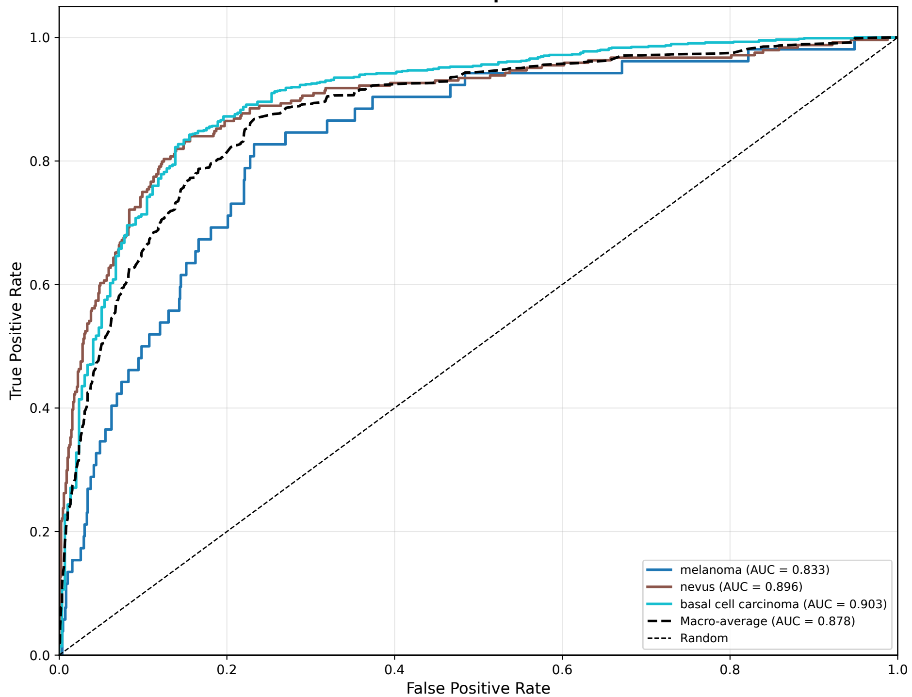
ROC Curves - padufes20
