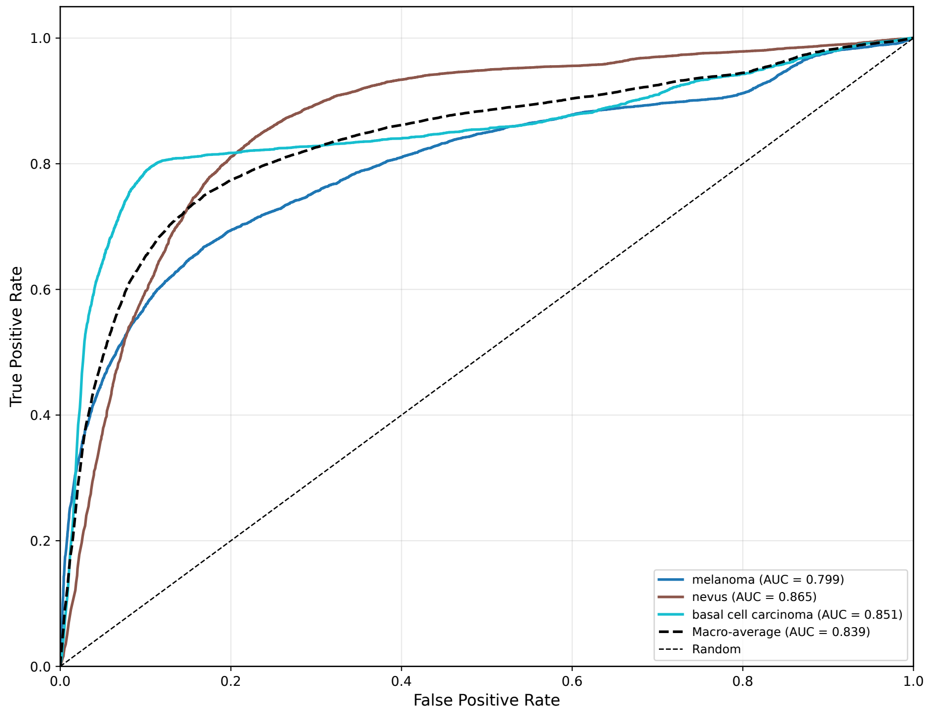
ROC Curves - isic2019
