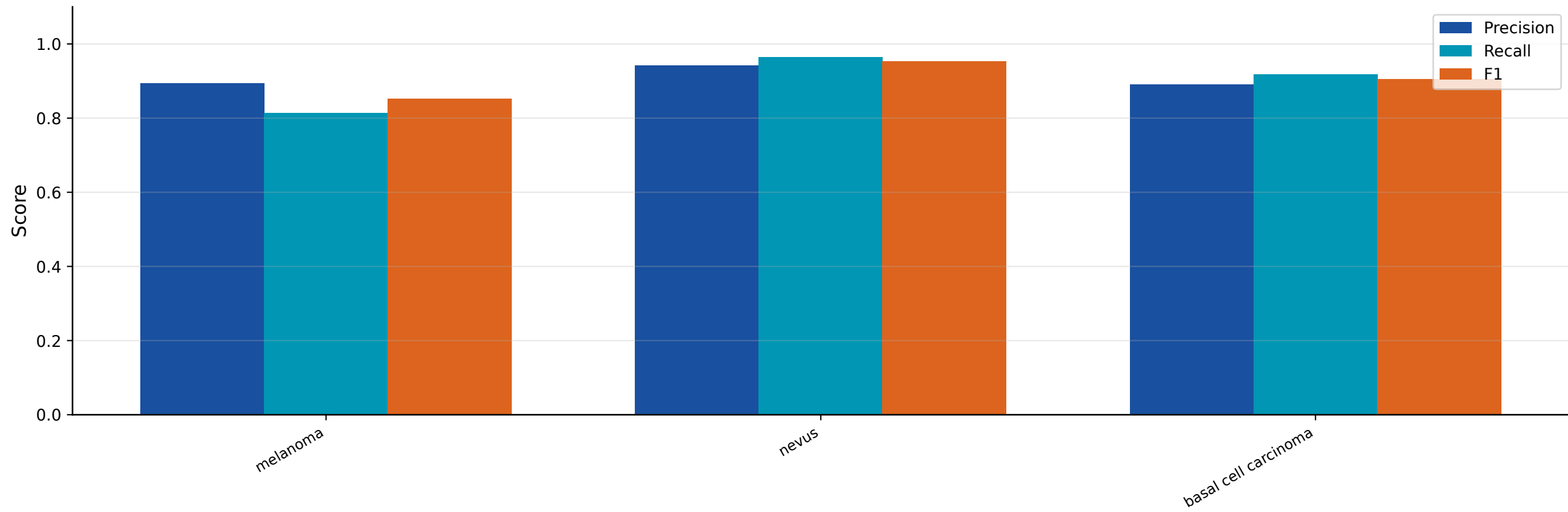
Per-Class Metrics - Test
