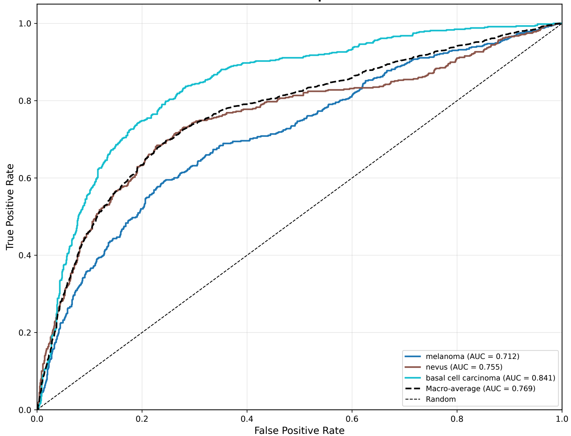
ROC Curves - fitzpatrick17k
