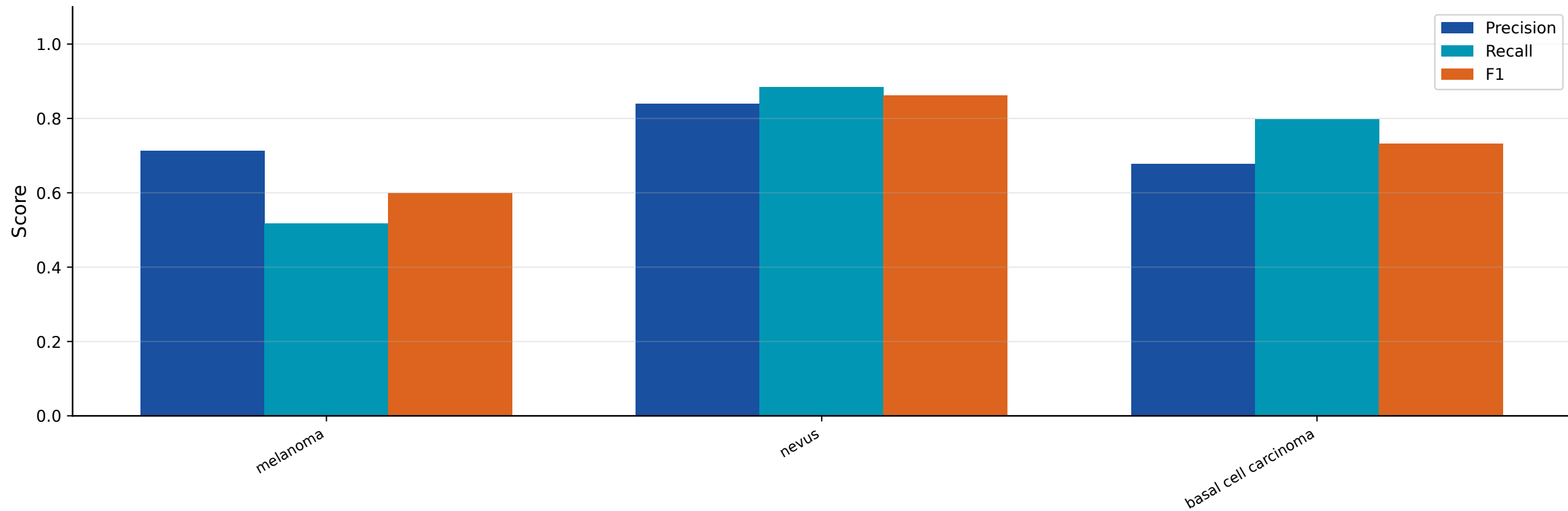
Per-Class Metrics - isic2019
