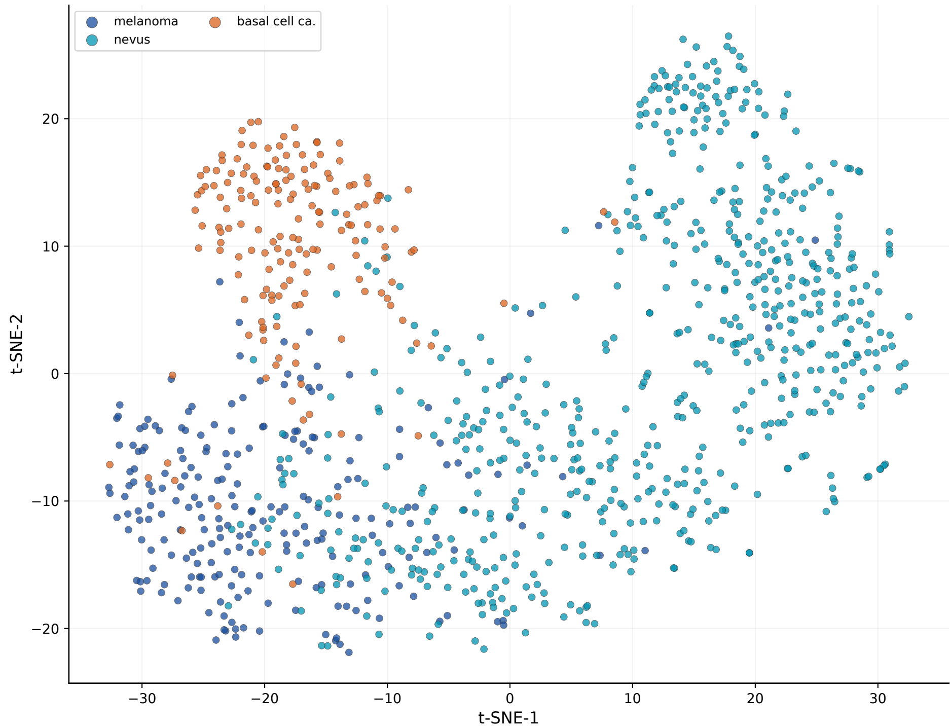
t-SNE - Test Set (RESM ResNet-18)
