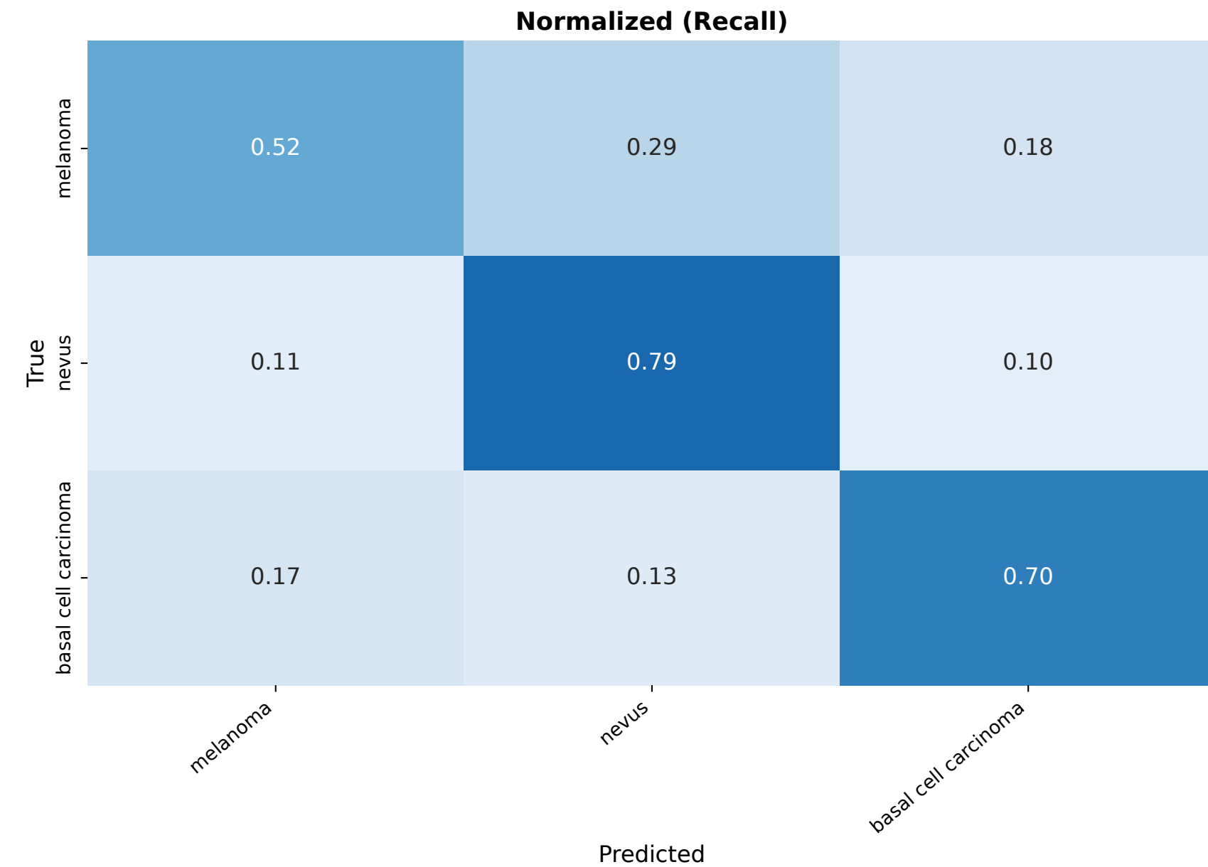
Confusion Matrix - isic2019
