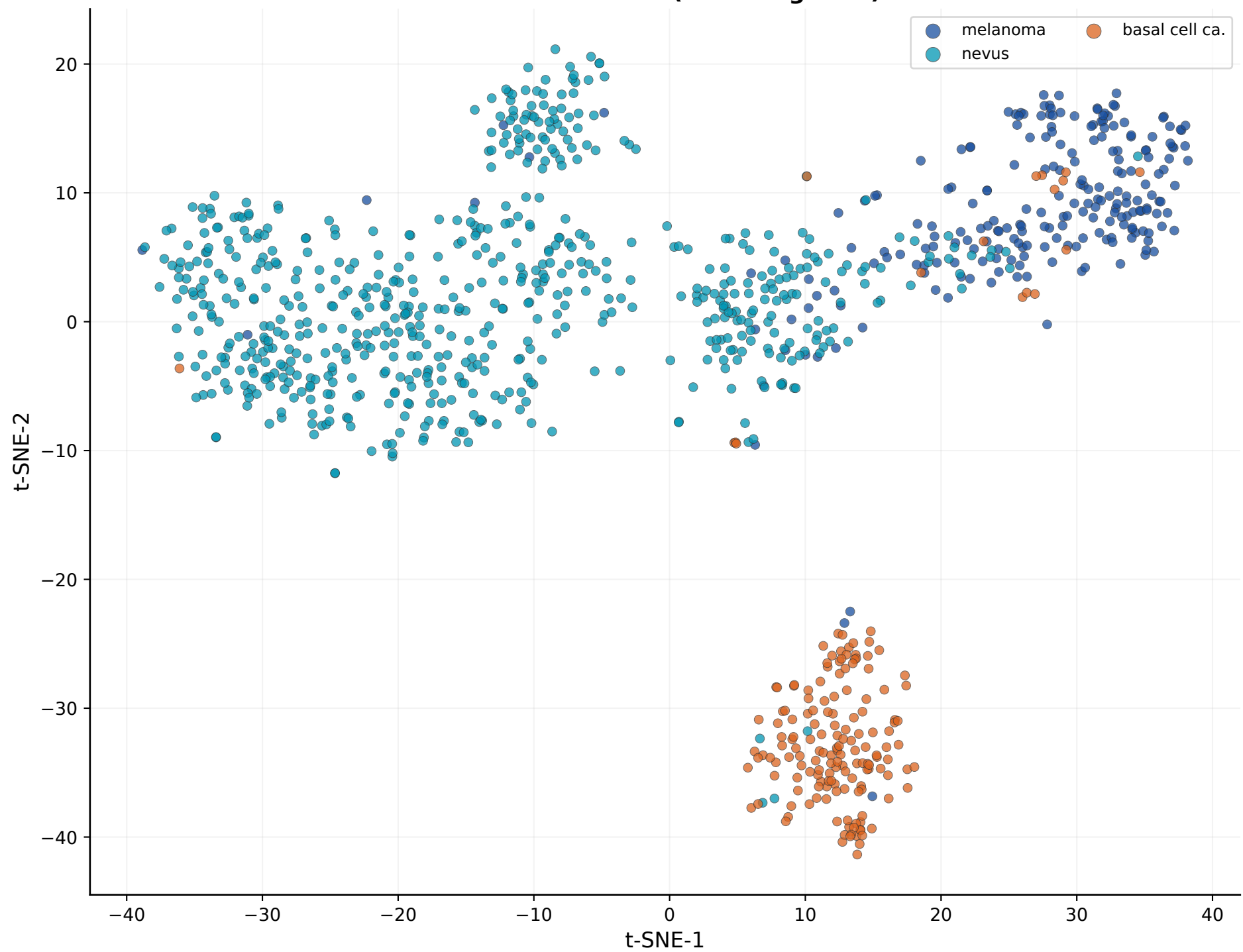
t-SNE — Test Set (PatchAlign ViT)
