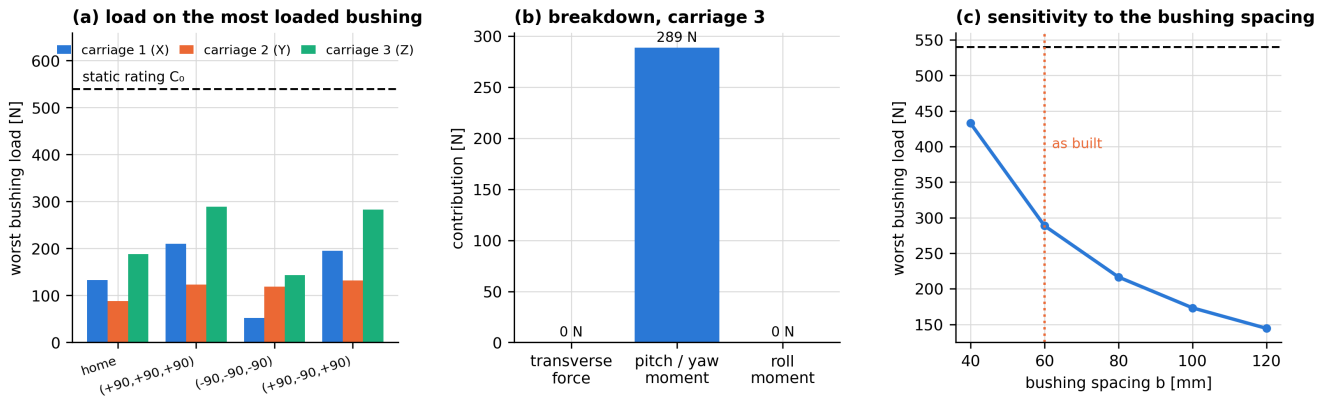
Figure 7: Guide verification: load on the most loaded bushing of each carriage, where that load comes from, and how it depends on the bushing spacing.
