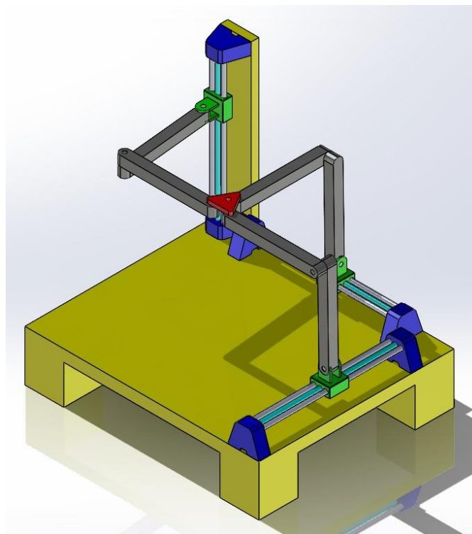
Figure 6: Final concept: welded frame, three orthogonal screw-driven axes, Tripteron legs and a spindle mounted on the moving platform.
