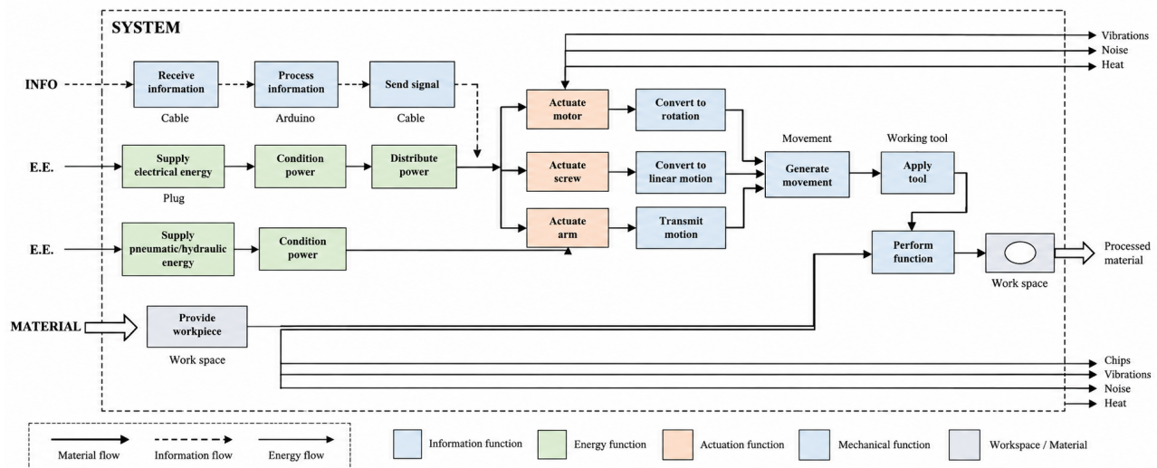
Figure 2: Functional structure of the machine: the material, energy and information flows and the elementary functions that transform them.
