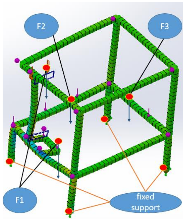
Applied forces and fixed supports
