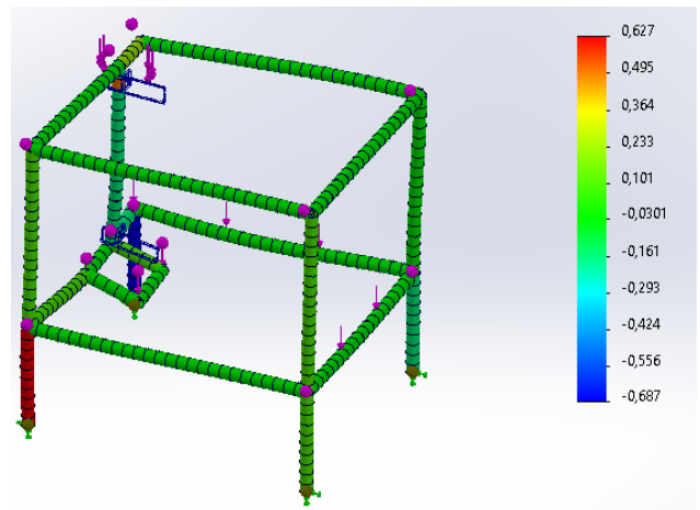
Shear stress, direction 2 [MPa]
