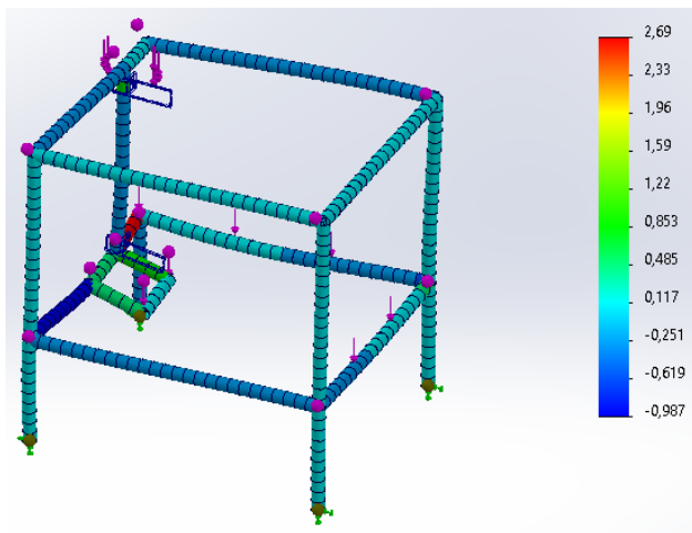
Shear stress, direction 1 [MPa]
