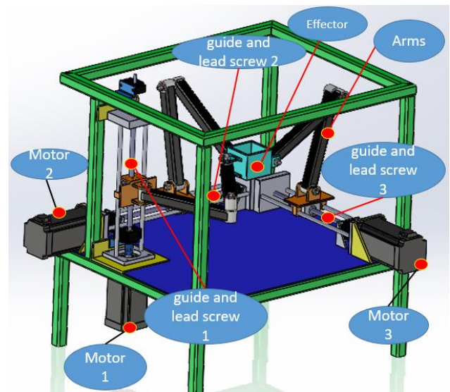
Components whose weight loads the frame
