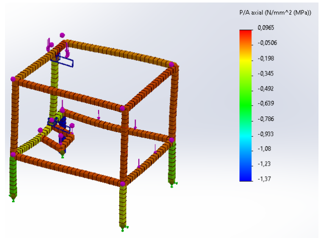
Axial stress [MPa]
