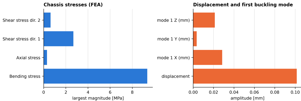
Figure 11: Range of each exported quantity and the resulting margins.
