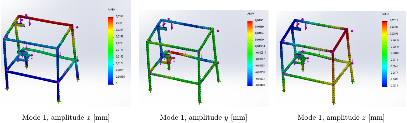
Figure 10: First buckling mode of the frame: a lateral sway of the uprights.
