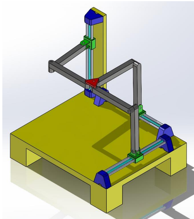
Figure 4: Final concept: welded frame, three orthogonal screw-driven axes, Tripteron legs and a spindle mounted on the moving platform.
