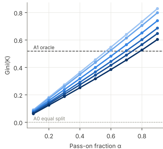
Sincere SOFA against \alpha ( \omega = 0.3 ); mean and 95 % interval over 50 seeds
