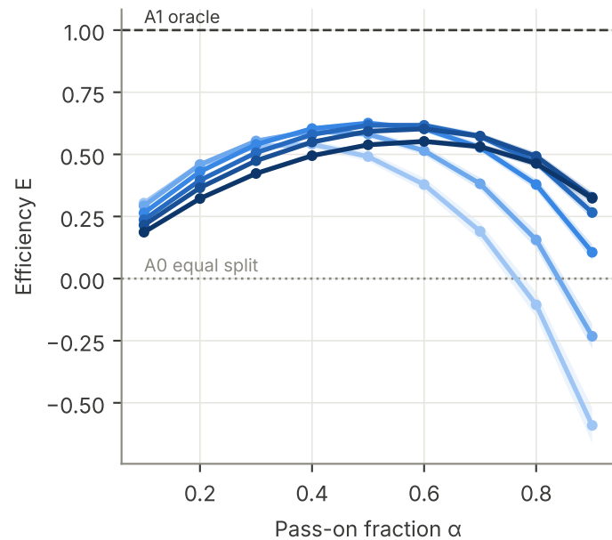
Sincere SOFA against \alpha ( \omega = 0.3 ); mean and 95 % interval over 50 seeds
