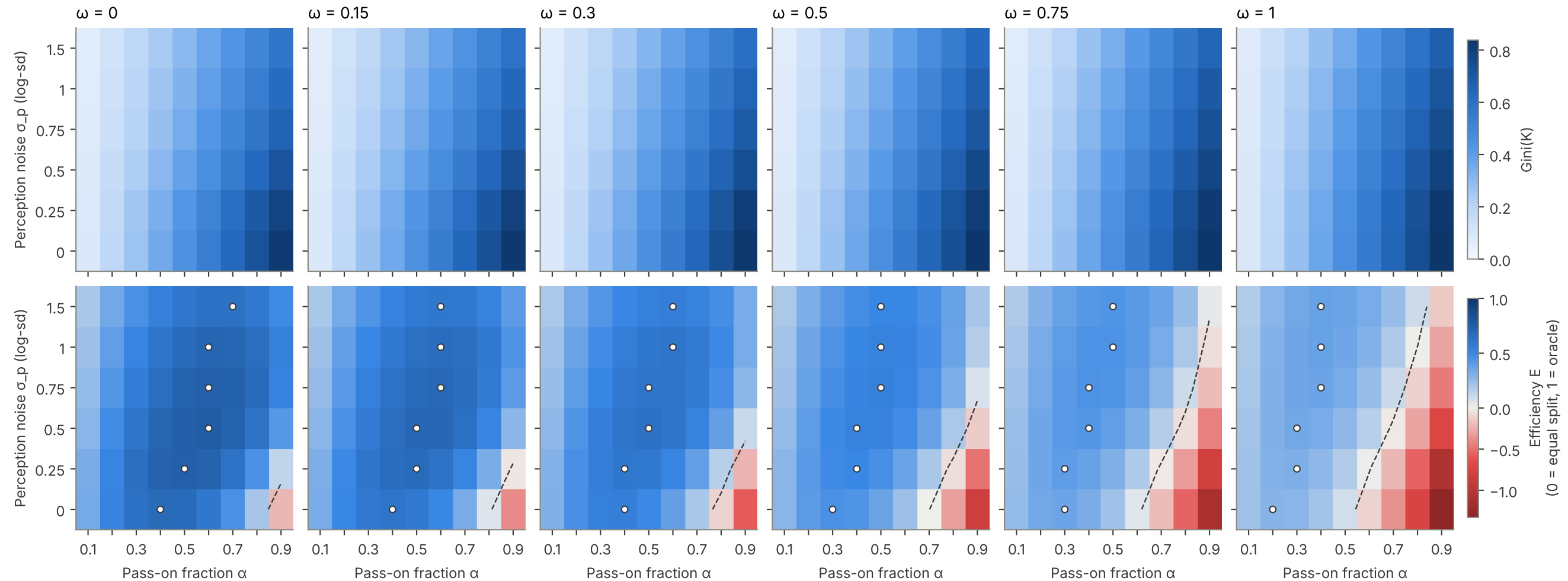
Sincere SOFA: concentration (top) and allocative efficiency (bottom); N = 500 , mean over 50 seeds. White dots: E-maximising \alpha per row; dashed: E = 0 .
