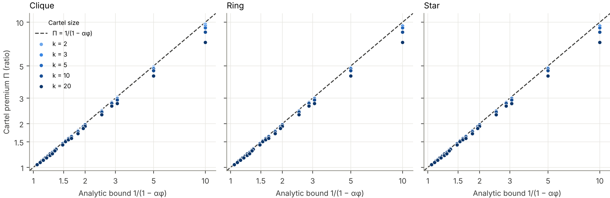
Cartel premium in the full model vs analytic bound (N = 500; mean over 50 seeds)
