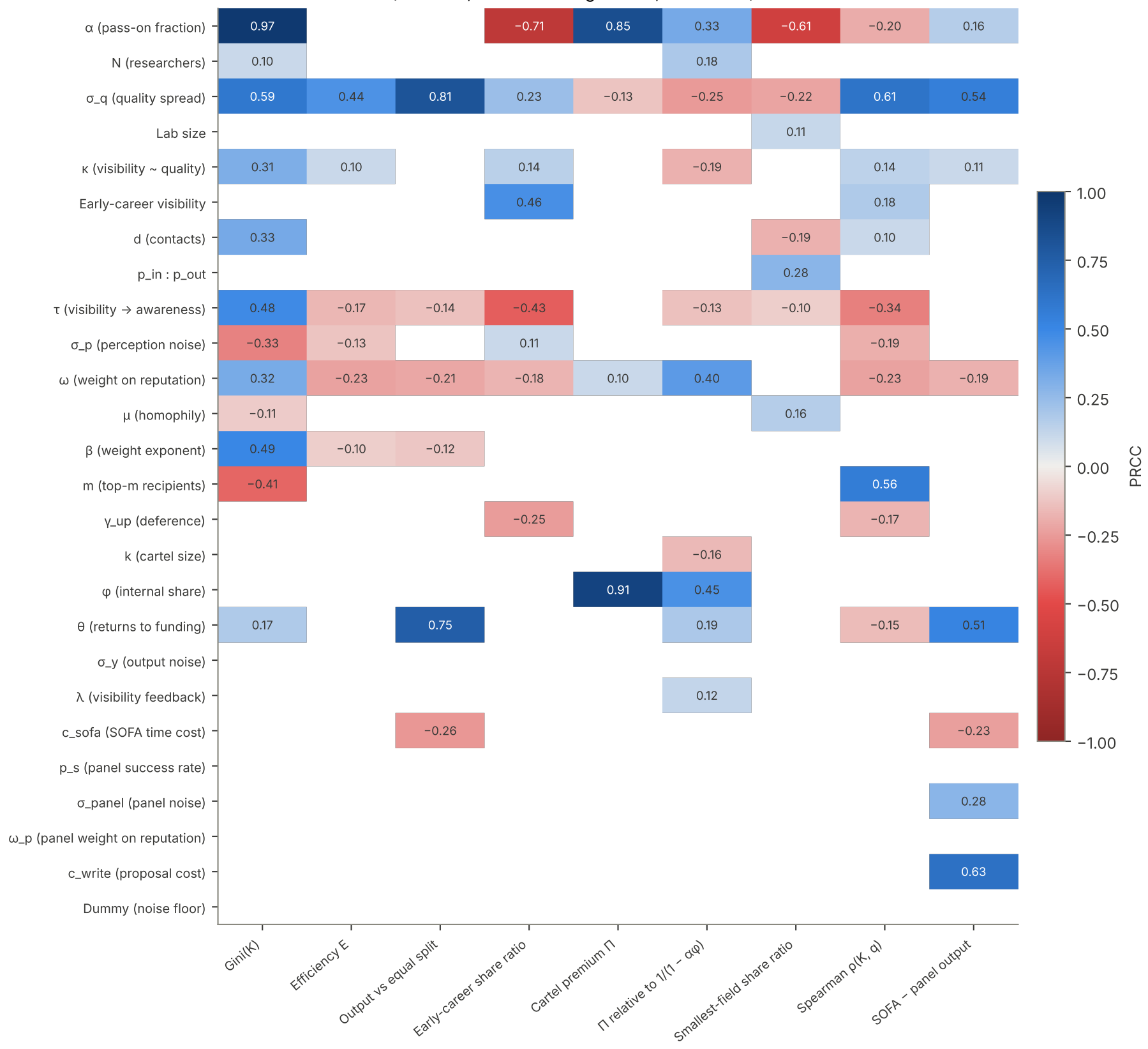
E7 mechanics: PRCC (n = 1000; blank = not significant, Bonferroni)
