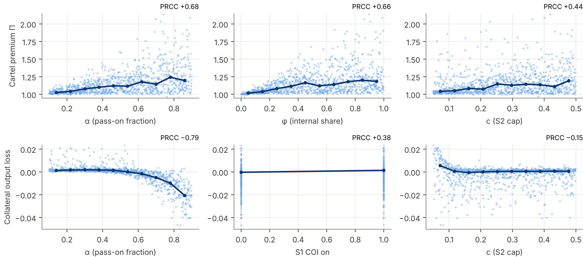
E7 safeguards: outcomes against their strongest (or selected) factors (dots = samples; line = median by factor decile)
