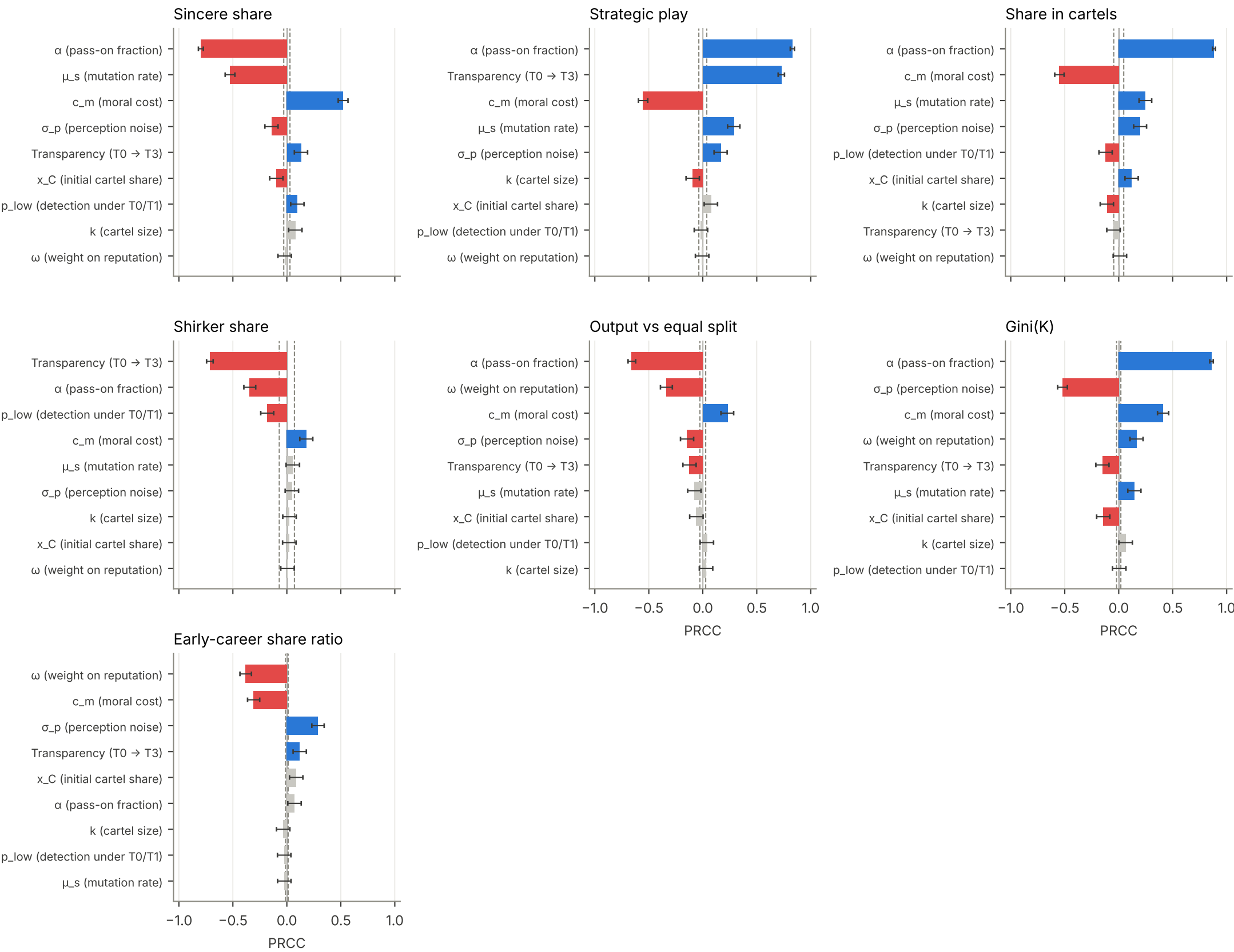
E7 evolution: Evolution of strategies (imitation, mutation, shirking) — PRCC, top 10 factors (n = 1000 samples; grey = not significant, Bonferroni; dashed = ± dummy)
