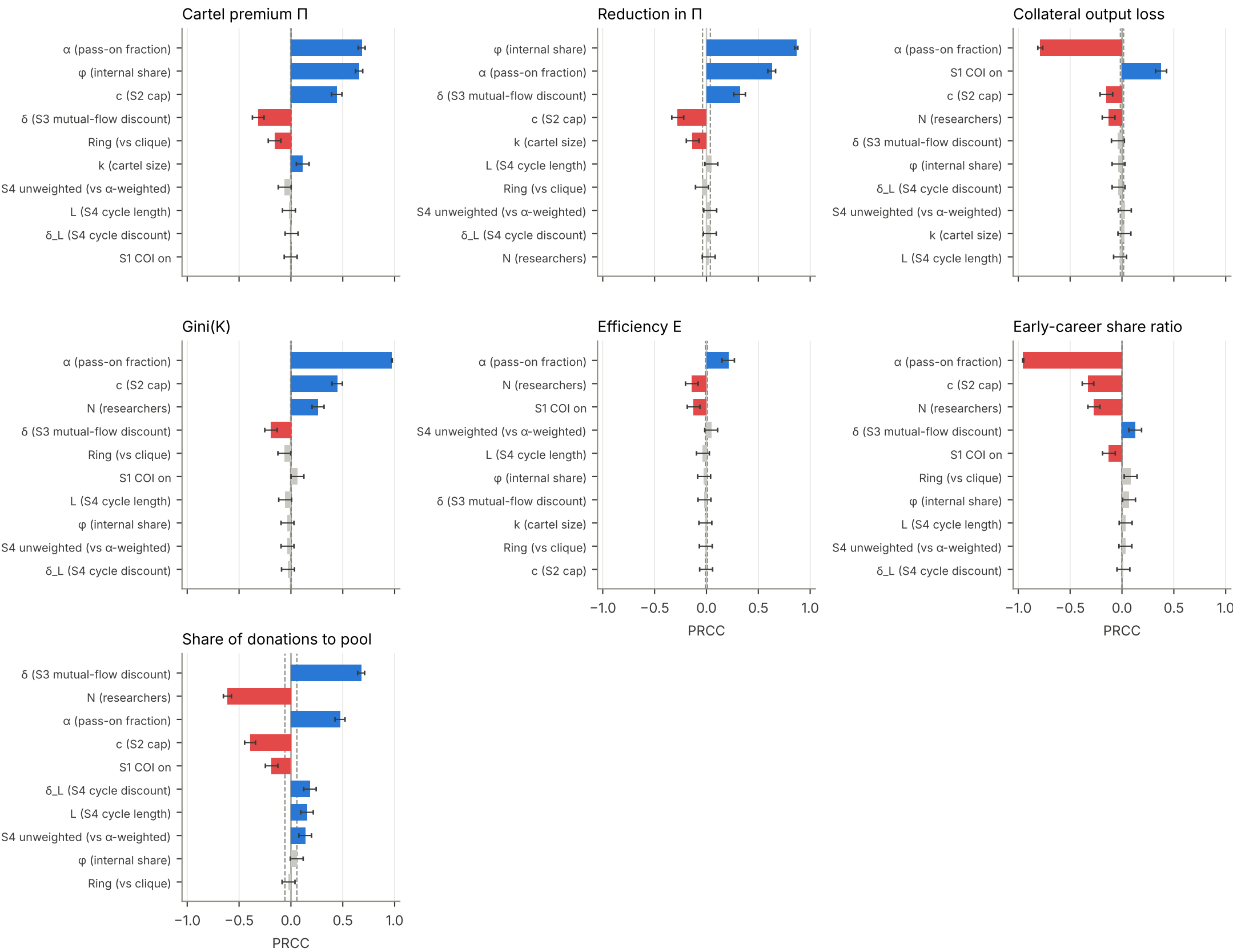
E7 safeguards: Safeguards S1–S4 against one cartel (static, solved) — PRCC, top 10 factors (n = 1000 samples; grey = not significant, Bonferroni; dashed = ± dummy)
