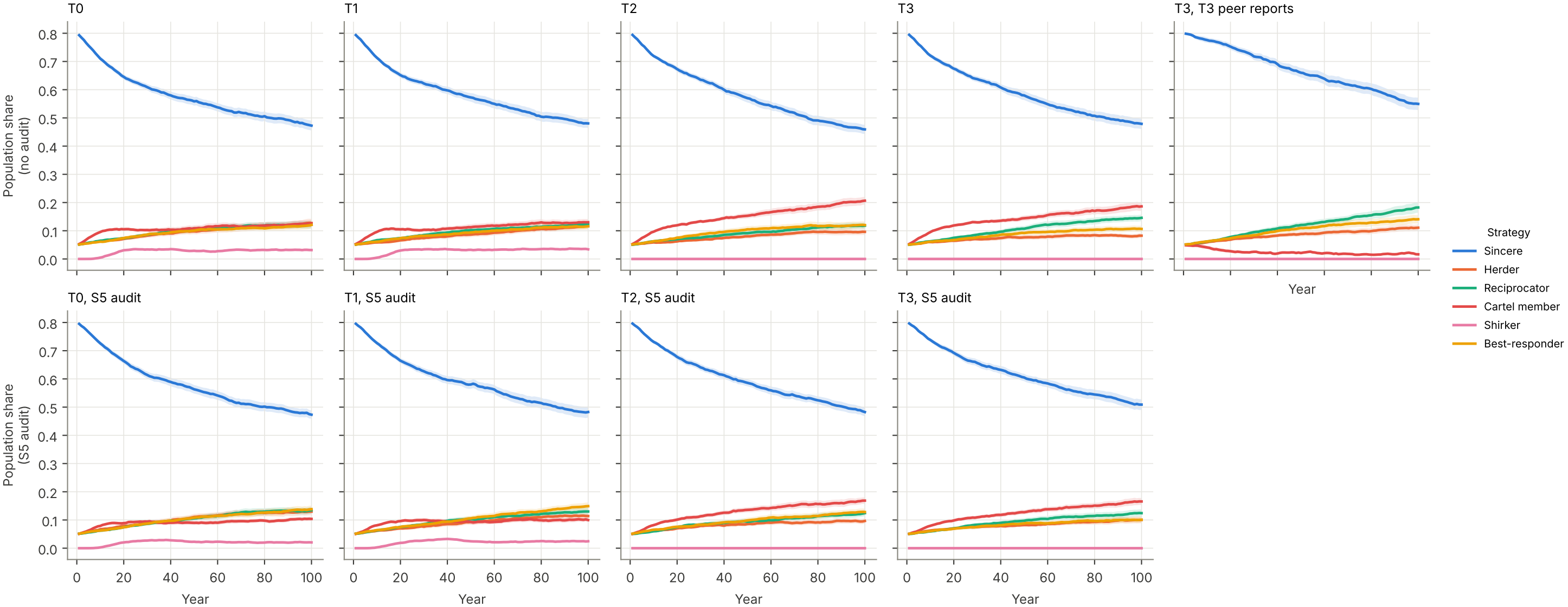
Evolution of strategies under imitation ( c_m = 0.05 ; mean and 95 % interval over 50 seeds)
