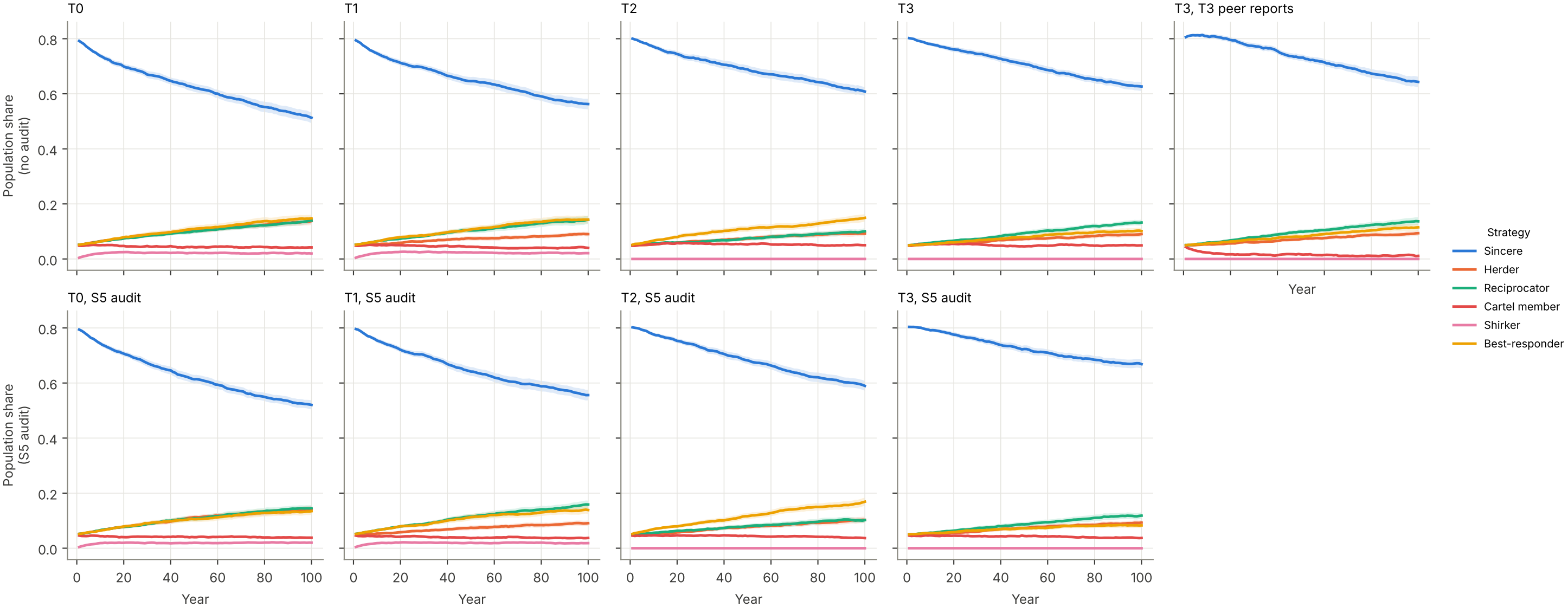
Evolution of strategies under imitation ( c_m = 0.2 ; mean and 95 % interval over 50 seeds)
