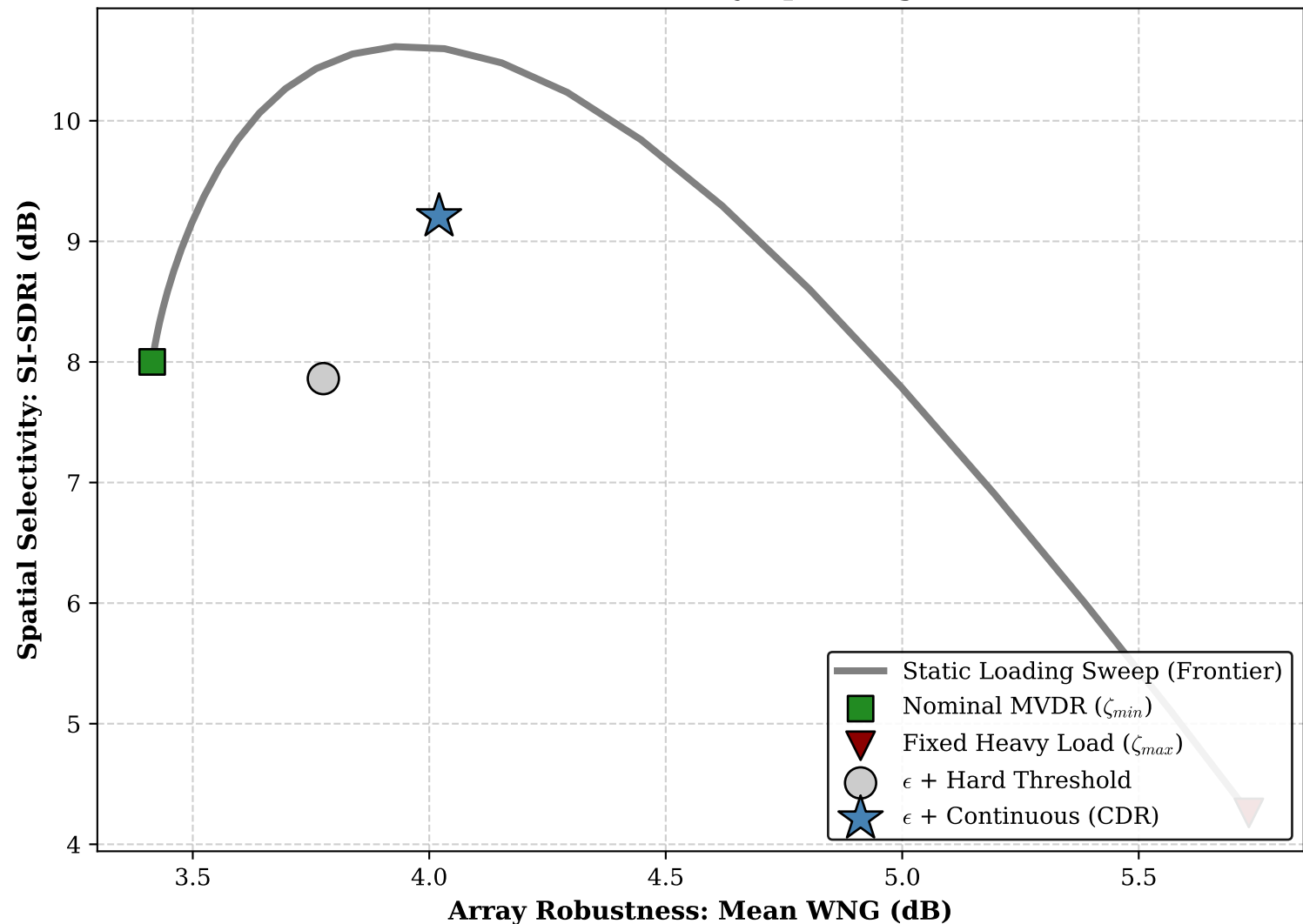
Robustness vs. Selectivity Operating Frontier
