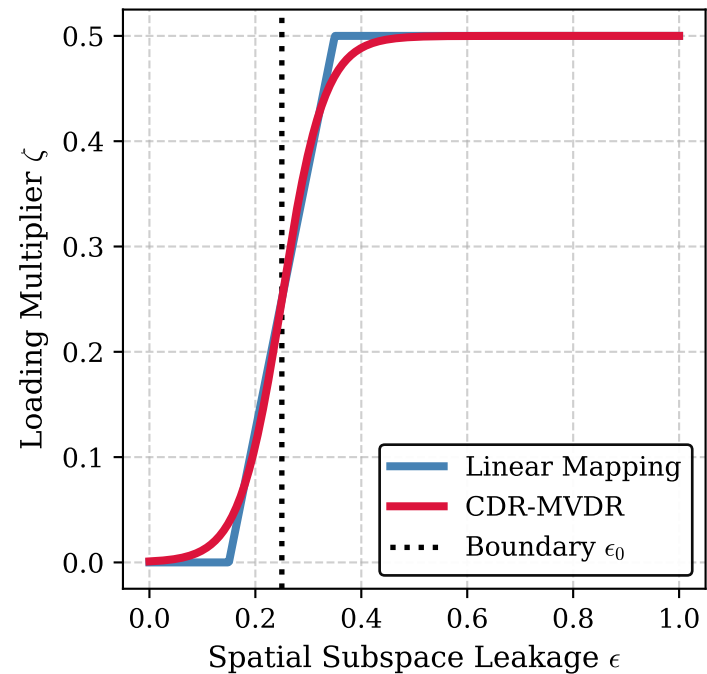
(a) \epsilon -to- \zeta mappings
