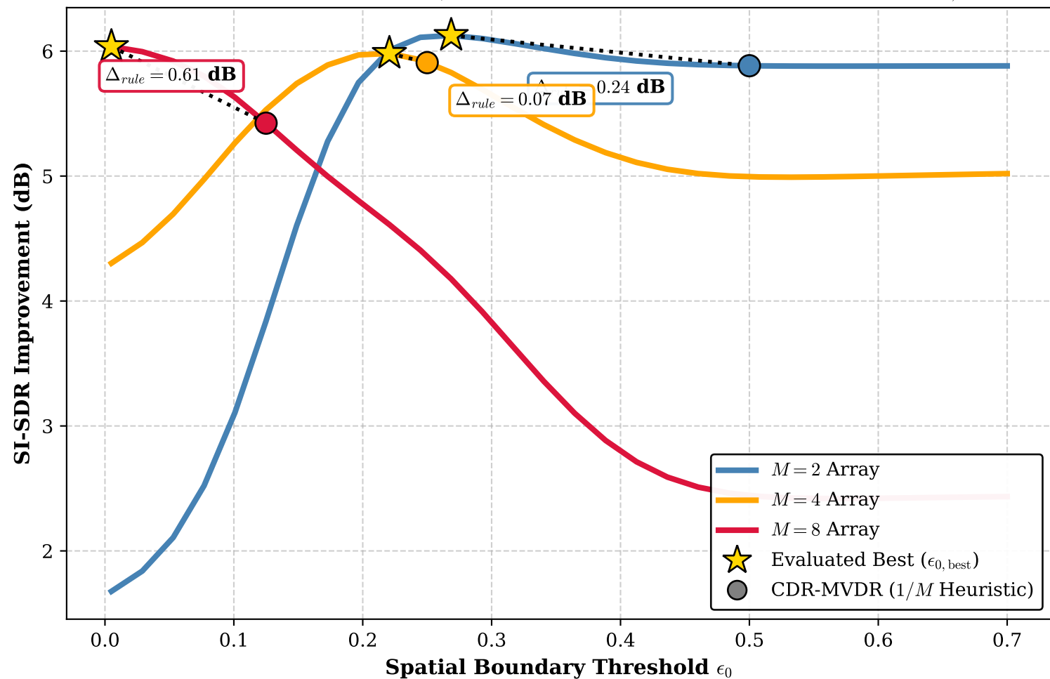
CDR-MVDR Oracle Gap: 1/M Transition Rule vs. Evaluated Best ( \epsilon_{0, \text{best}} )
