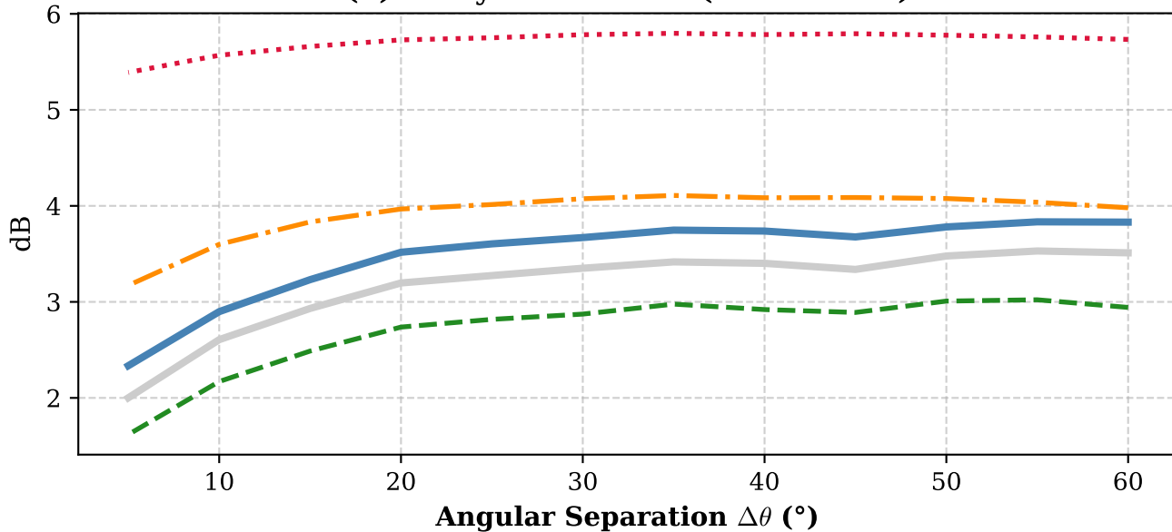
(b) Array Robustness (Mean WNG)
