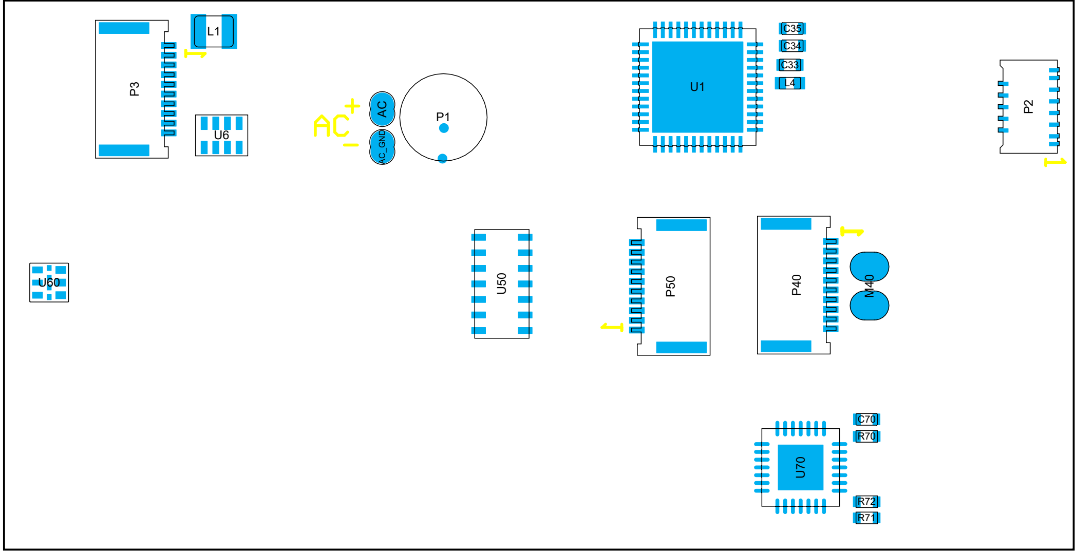
View from Bottom side (Scale 5:1)
