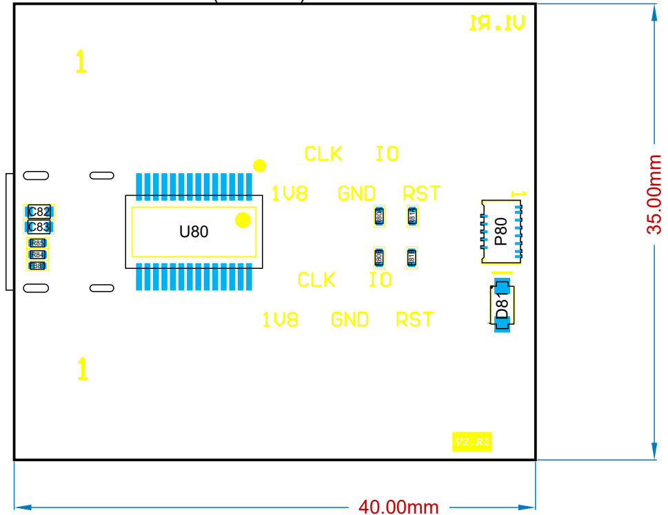
View from Bottom side (Scale 5:2)
