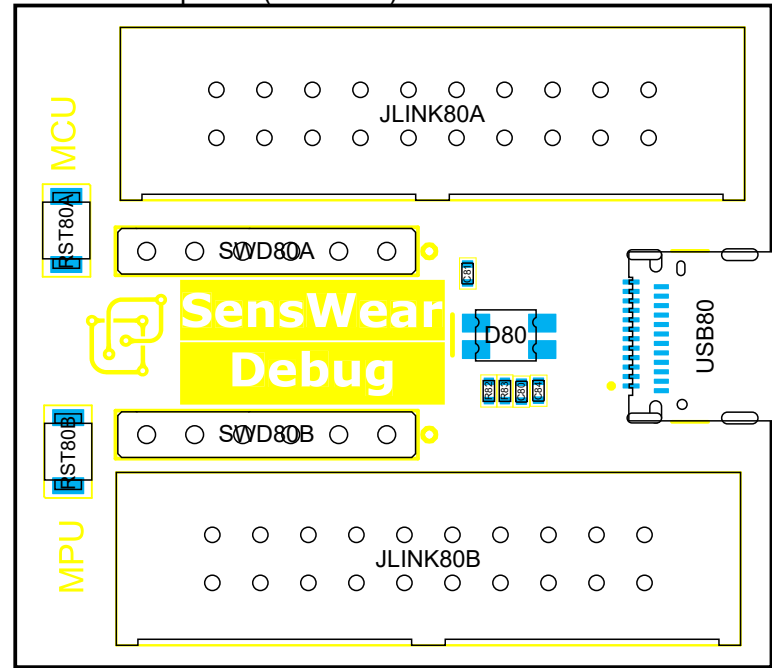
View from Top side (Scale 5:2)
