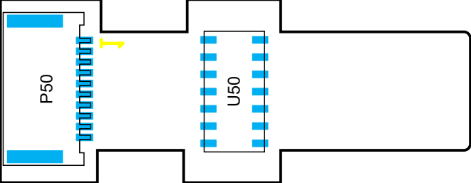
View from Bottom side (Scale 4:1)
