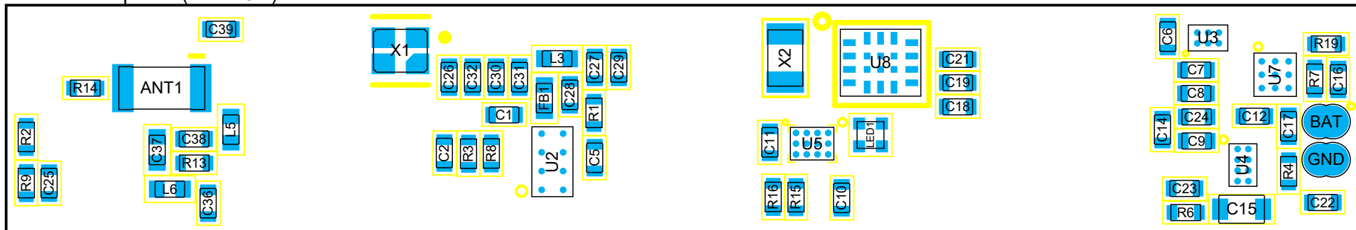
View from Top side (Scale 5:1)
