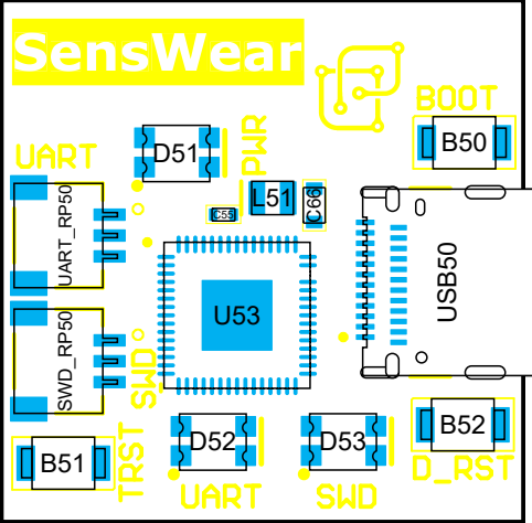
View from Bottom side (Scale 5:2)
