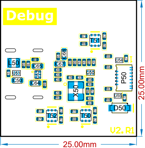
View from Bottom side (Scale 5:2)
