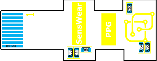
View from Top side (Scale 4:1)
