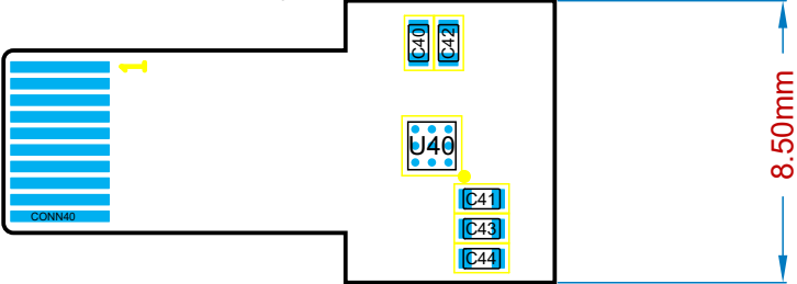
View from Top side (Scale 4:1)
