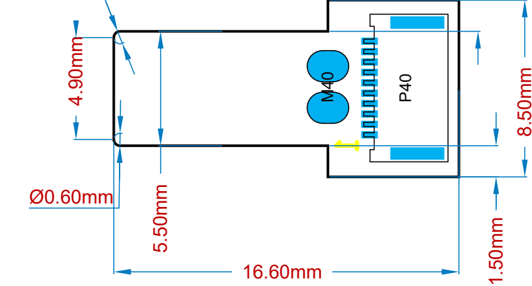
View from Bottom side (Scale 4:1)
