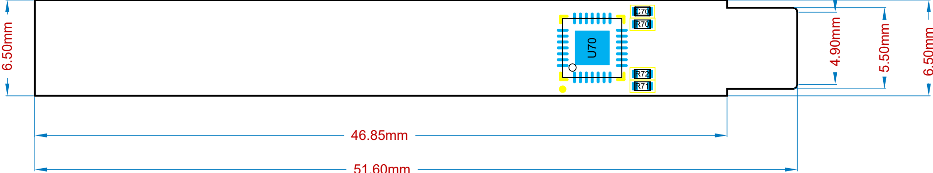
View from Bottom side (Scale 4:1)
