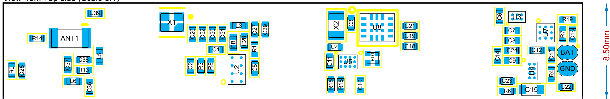
View from Top side (Scale 5:1)
