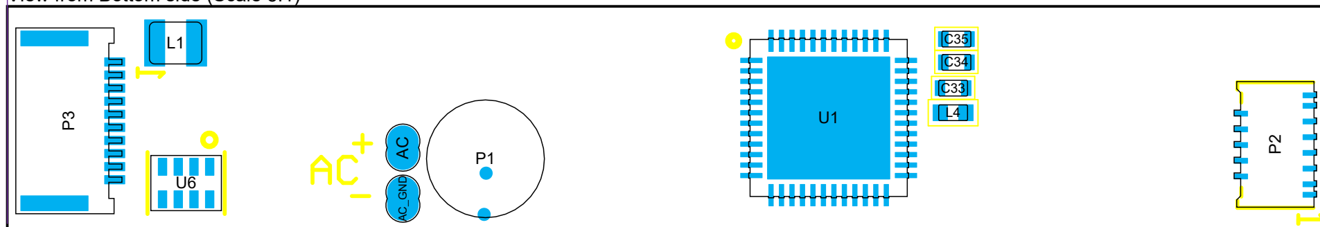
View from Bottom side (Scale 5:1)
