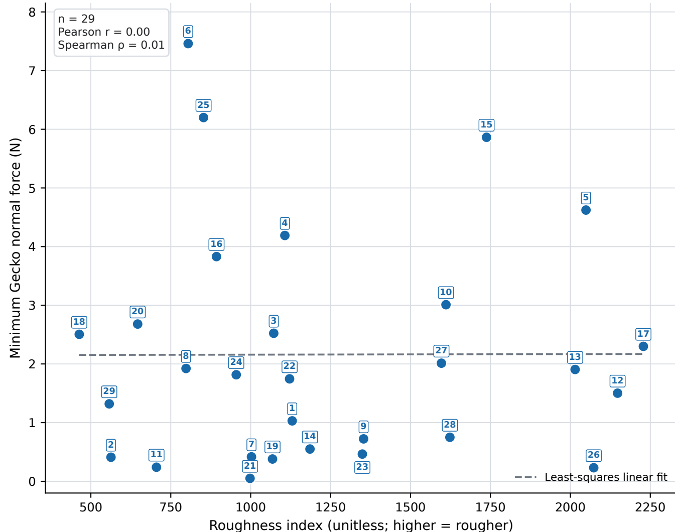
MatForceFinal: roughness index versus Gecko force
