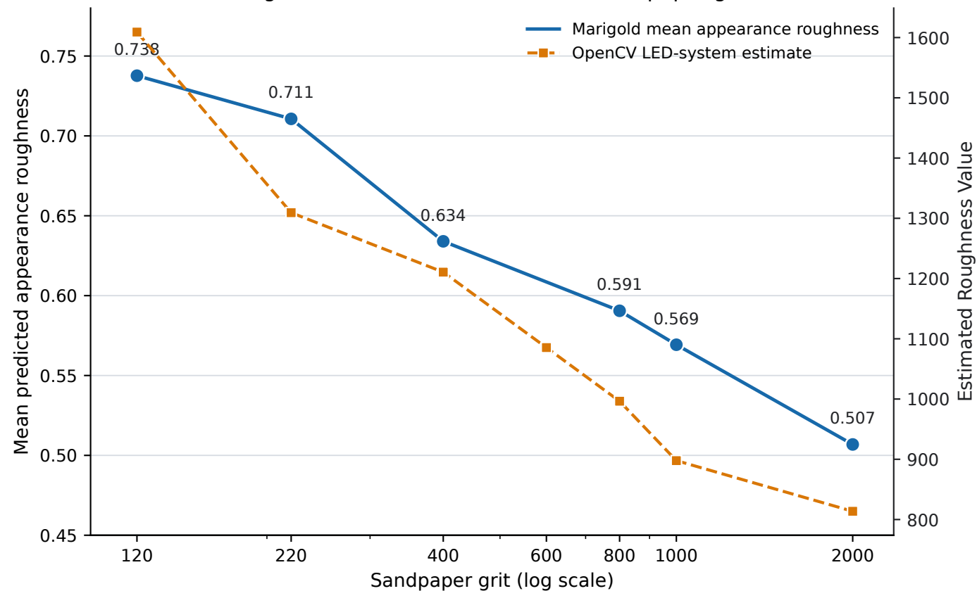
Roughness Detection Values across sandpaper grits
