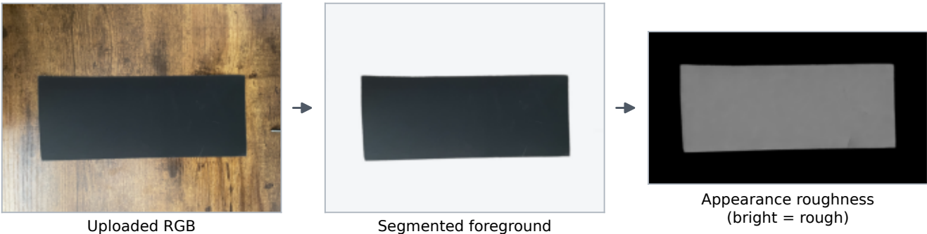
Grit 2000 | mean = 0.507
