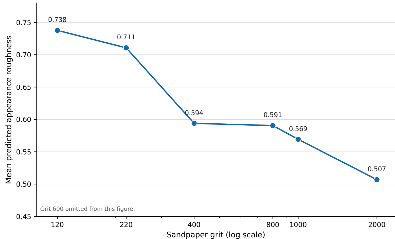
Marigold appearance roughness across sandpaper grits
