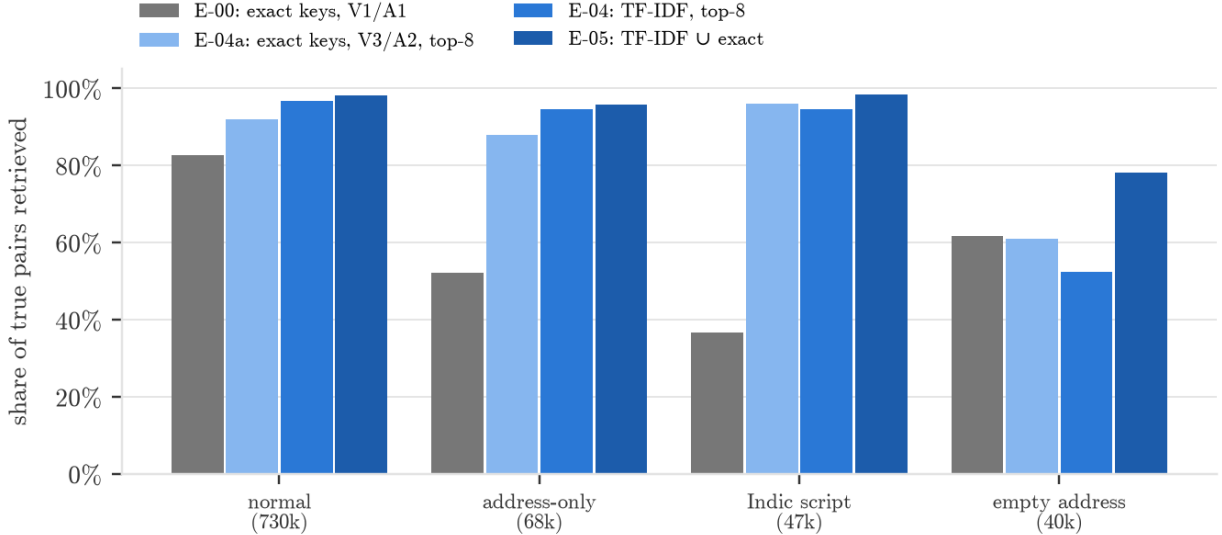
Figure 3: Share of true pairs retrieved, by type of positive (DEV-VAL). Counts are true pairs of each type.
