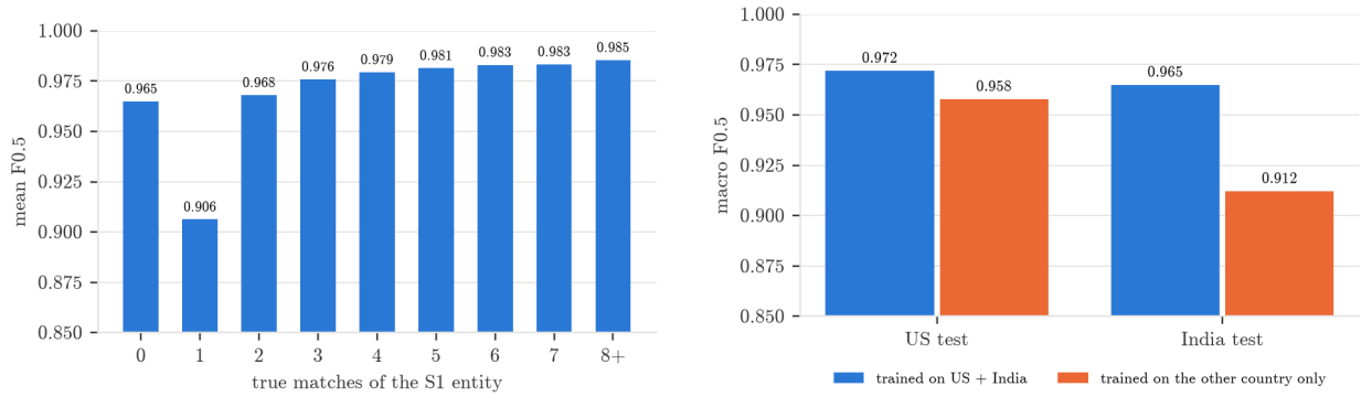
Figure 9: Left: mean F_{0.5} by number of true matches (DEV-VAL). Right: transfer between countries (Section 11).
