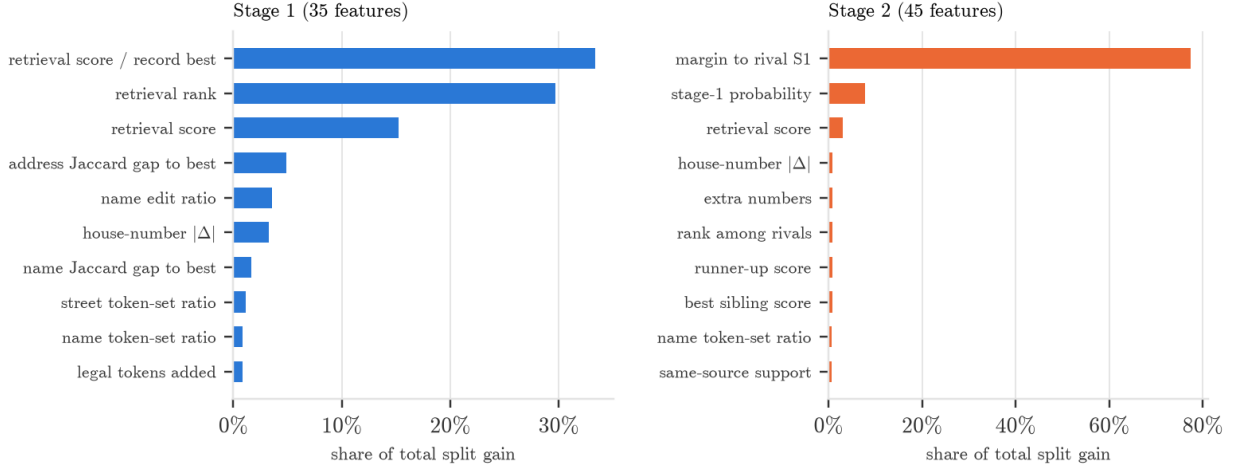
Figure 4: Share of total split gain per feature, top ten per stage.
