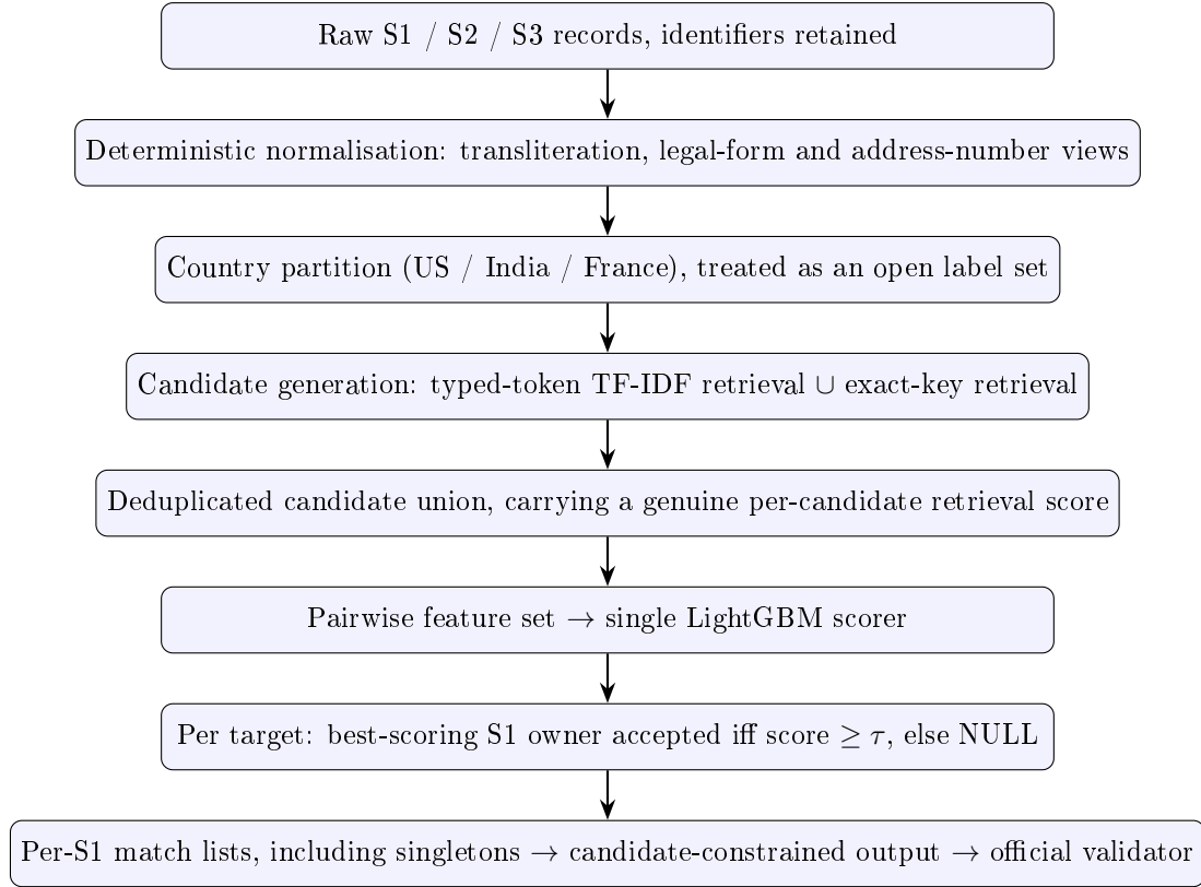
Figure 1: End-to-end pipeline of the submitted system. Only Stage 1 pairwise scoring is used; a candidate entity-level second stage was implemented, tested, and excluded (Section 7).
