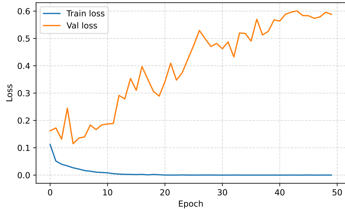
Training / Validation Loss
