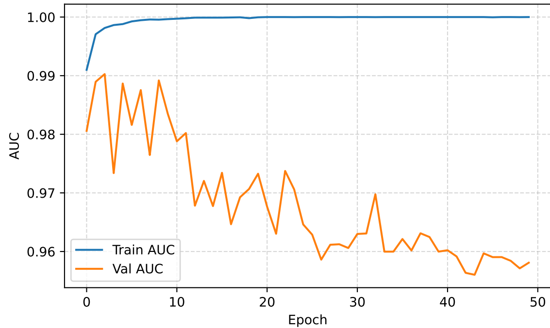
Training / Validation Area Under Curve (AUC)
