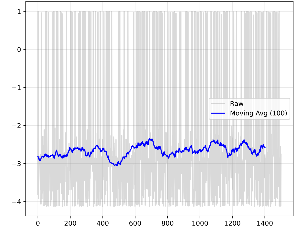
Training Rewards
